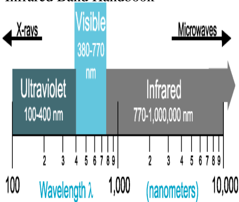
Fig. 1.1 The optical portion of the electromagnetic spectrum
