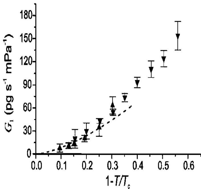
FIG. 1. The quantity G_1 plotted as a function of (1 - T/T_c) .
